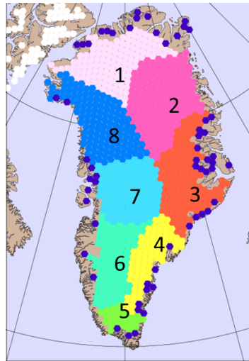
Figure 5.1: Overview of the drainage basin definition and the solution area. Ellesmere Island is shown in white and GIS surrounding glaciers and ice caps in dark violet.
