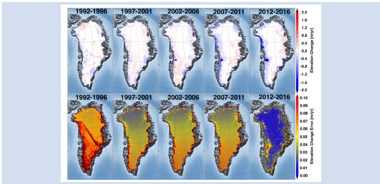
Figure 2.3: Examples of SEC grids and their associated error grids. from Sørensen et al., (2018b).
