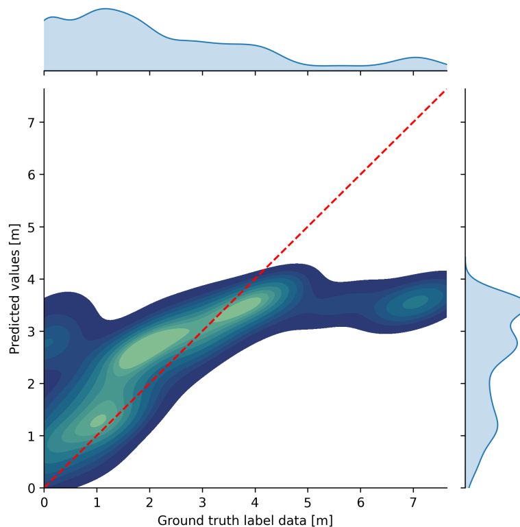
Figure 7.1: Density scatter plot and frequency density (top + right) for SGL depth prediction vs ground truth. Frequency shown in ranges from blue to green.
