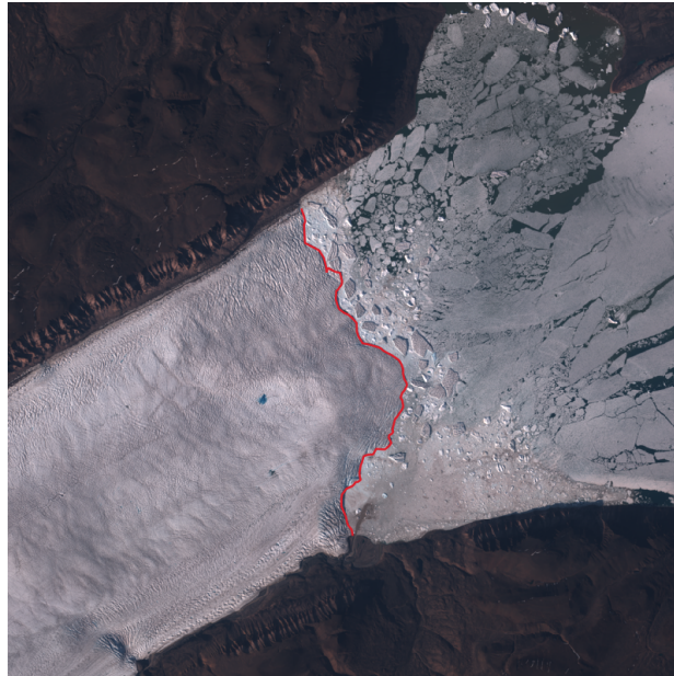
Figure 8-1: Example CFL of the Hagen glacier
