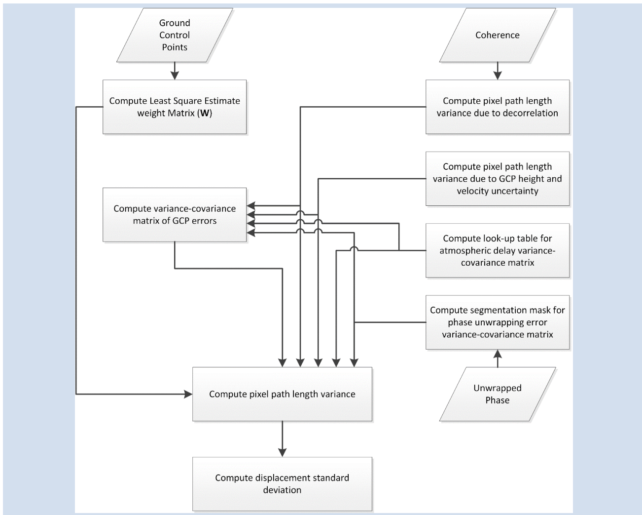
Figure 3.1: Error prediction framework for interferometric displacement measurement.
