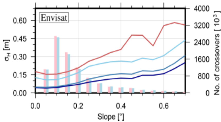
Figure 2.1: Crossover statistics of Envisat over Antarctica from Schröder et al. (2019). Standard deviation as a function of slope. The curves represent different retrackerers employed to the data and the vertical bars indicate number of crossovers.
