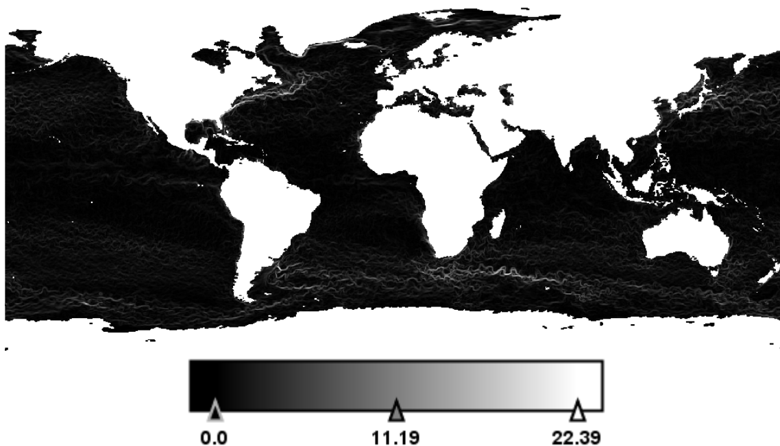
Figure 12. The combined Sobel North and West filters showing regions with high local horizontal gradients.
