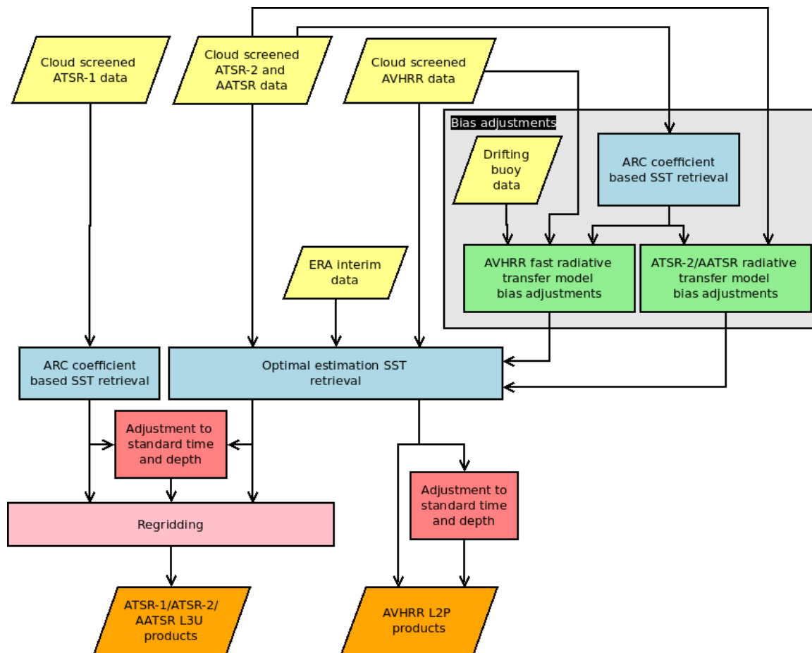
Figure 16. Overview of the processing of ATSR- and AVHRR-series data to produce the output data files for the long term ESA SST CCI products. ATSR-1 SSTs are retrieved using a coefficient based approach; ATSR-2, AATSR and AVHRR series SSTs are retrieved using optimal estimation. The optimal estimation approach requires bias corrections for the fast radiative transfer model that is used; these are calculated using ATSR-2 and AATSR SSTs calculated using a coefficient based retrieval. Yellow boxes denote input data; blue shows SST retrieval steps; green are bias adjustment calculations; red indicates adjustment of SSTs to standard time and depth using a diurnal variability model; pink is used where the full resolution ATSR series data are regridded; orange are the output ESA SST CCI products.
