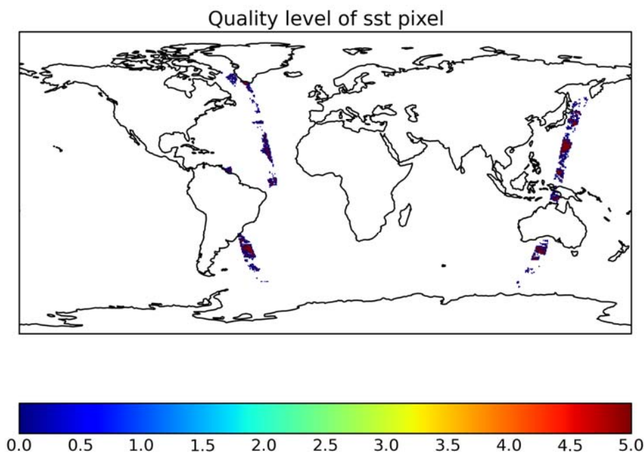
Figure 15. Quick plot of the quality_level variable from a L3U file. Only values of 0 (blue) and 5 (red) are used in the ESA SST CCI files.
