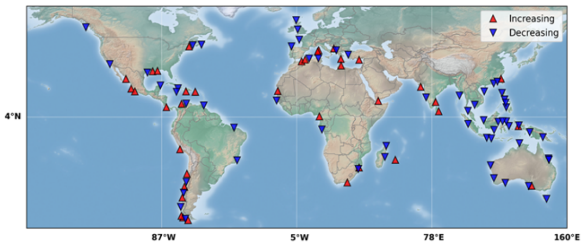
Figure 1: Coastal sea level sites where the trend nearby the coast differs from offshore (considered here at 15 km). Red/blue triangles correspond to trends that are either increasing/decreasing in the 4-5 km towards the coast.
