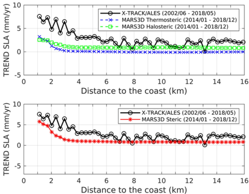
Fig.4: Comparison of the evolution, along the altimeter track over the first 16 km of the coast, of the X-TRACK/ALES SLA trend (calculated over the period June 2002 - May 2018) with : ( above ) that of the thermosteric and halosteric component ; and ( below ) that of the steric component (calculated over the period January 2014 - December 2018 and estimated using temperature and salinity data from the MARS3D model) for site 085/03 near the coast of Senetosa.
