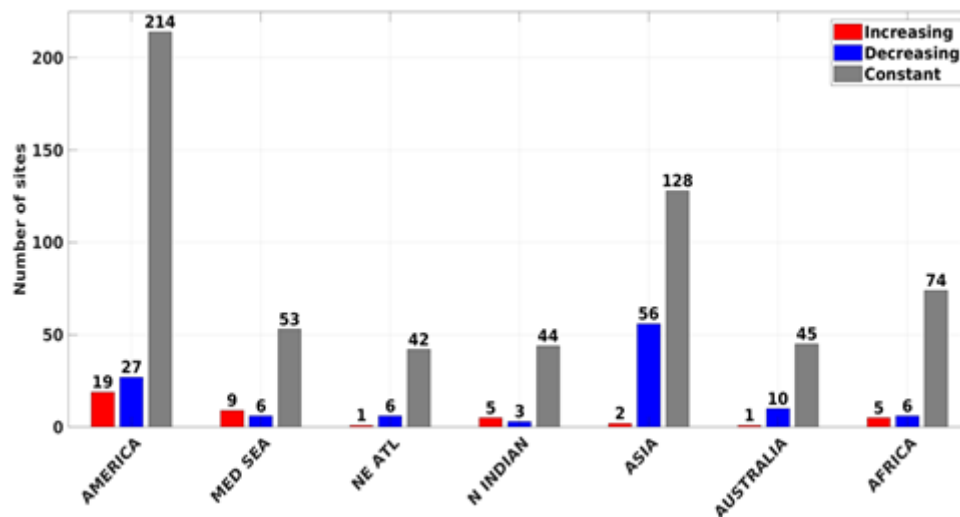
Figure 2: Coastal trend behaviors compared to offshore for the different studied regions. Grey/red/blue bars represent the number of constant/increasing/decreasing trends nearby the coast compared to offshore.
