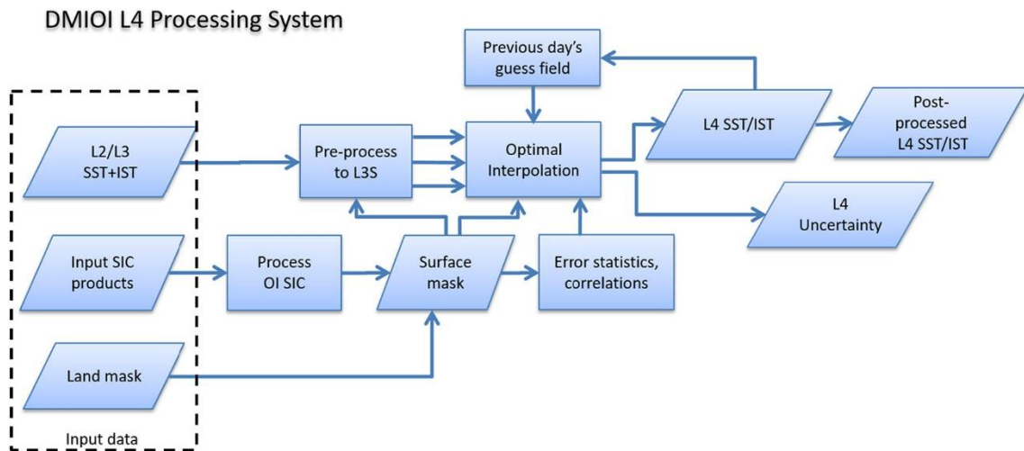
Figure 2-10: Schematic diagram illustrating the processing steps of the DMIOI L4 Processing System.
