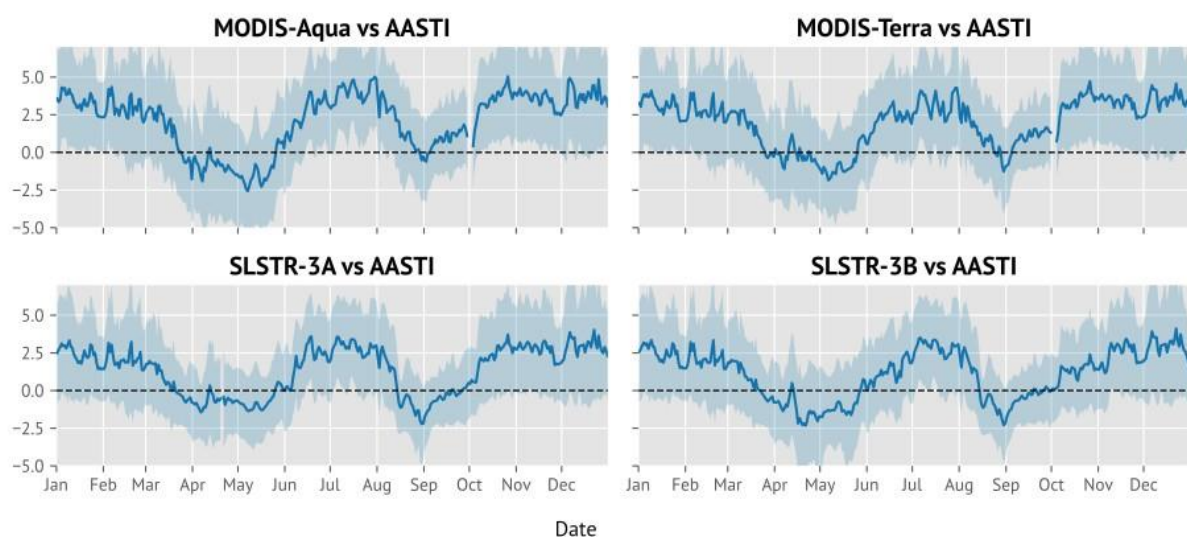
Figure 2-13: Time-series of mean daily biases between MODIS/Aqua and AASTI (top left), MODIS/Terra and AASTI (top right), SLSTR/S3-A and AASTI (bottom left) and SLSTR/S3-B and AASTI (bottom right) for 2021. Units of the Y-axis are in °C.
