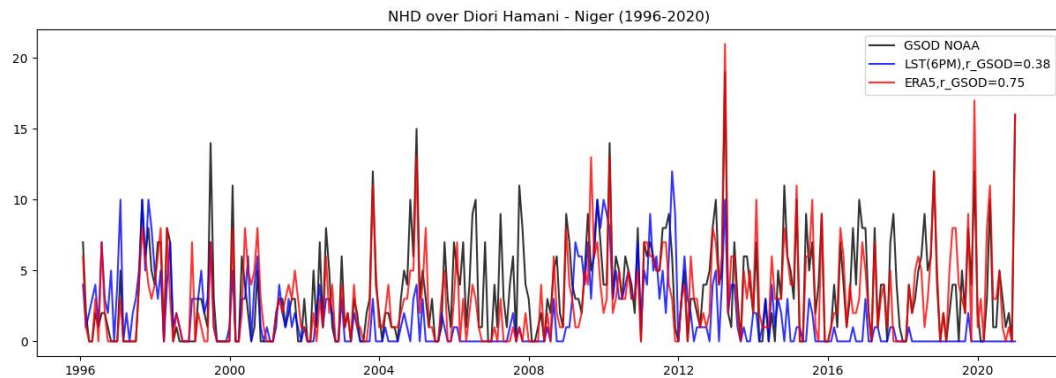
Figure 4-43: Monthly Number of Hot Days (NHD) over Diiori Hamani (Niger) station for the period 1996-2020
