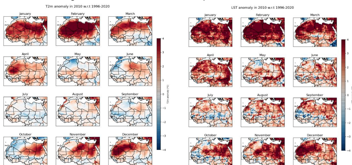
Figure 4-40: Monthly anomalies of Tx during 2010 with respect to the 1996-2020 baseline for ERA5 T2m (left) and MW LST_cci (right)
