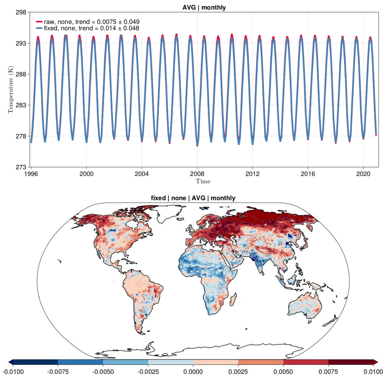
Figure 4-38: (Top) Time series of mean global monthly actual LST from the MW LST_cci product v2.33. The numerical values of the trends are also shown on the plot where ‘raw’ refers to the MW LST data without applying the LST correction for orbital drift and ‘fixed’ refers to the MW LST data where the orbital drift LST correction has been applied. (Bottom) Geographical distribution of trends in the actual MW LST monthly data where the orbital drift LST correction has been applied. Red indicates positive trends and blue negative trends in the data. The units of the trend are in K per month.
