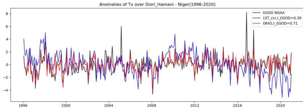
Figure 4-42: Monthly anomaly of maximum temperature (TX) over Diiori Hamani (Niger) station for the period 1996-2020
