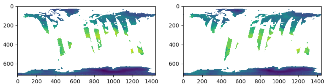
Figure 4-36: Example of the LST_cci MW LST product for a day in 1996 in ASC and DES mode. Some regions in Europe are covered twice by the swaths; but some other regions in Europe are not covered at all.
