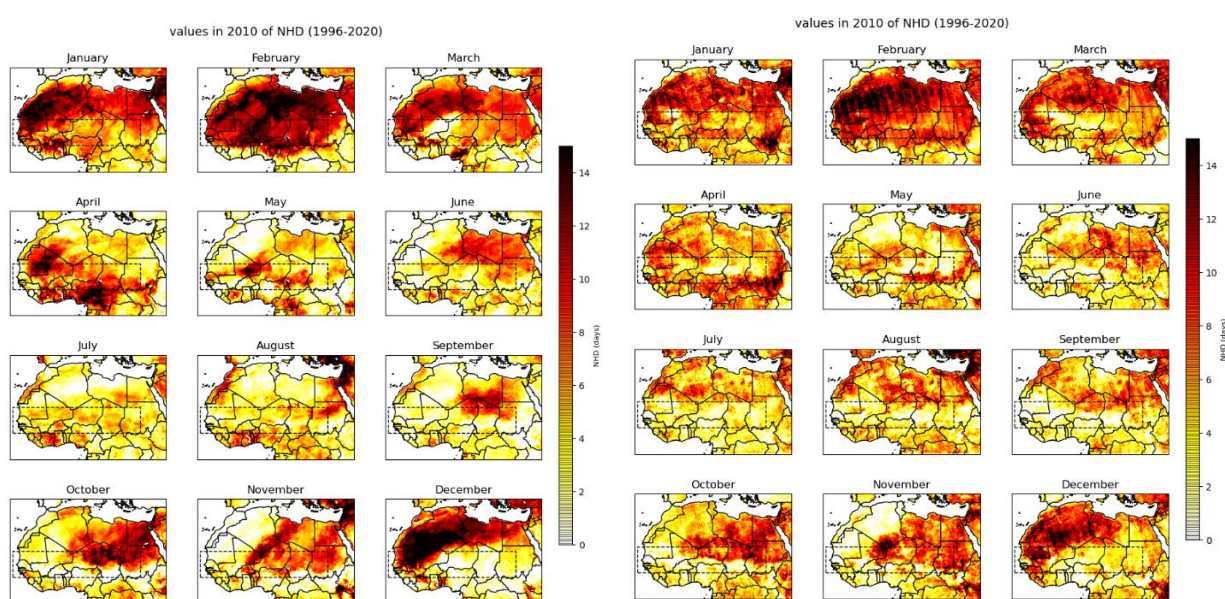
Figure 4-41: Monthly climatology of the Number of Hot Days (NHD) over the Sahel for the period 1996-2020 using ERA5 data (left) and using MW LST_cci data (right).
