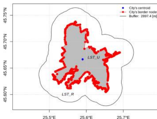
Figure 2-30: Delimitation of areas for computing LST_cci urban and LST_cci rural . The example is for Braşov City (Romania). The rural buffer is drawn at \frac{1}{2} \times average distance between the city centroid (blue dot) and nodes of the urban administrative perimeter (red dots).
