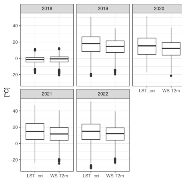
Figure 2-25: Summary statistics for LST_cci retrieved from L3C-LST-SLSTRB-0.01 and weather station air temperature (WS T2m) for each year.
