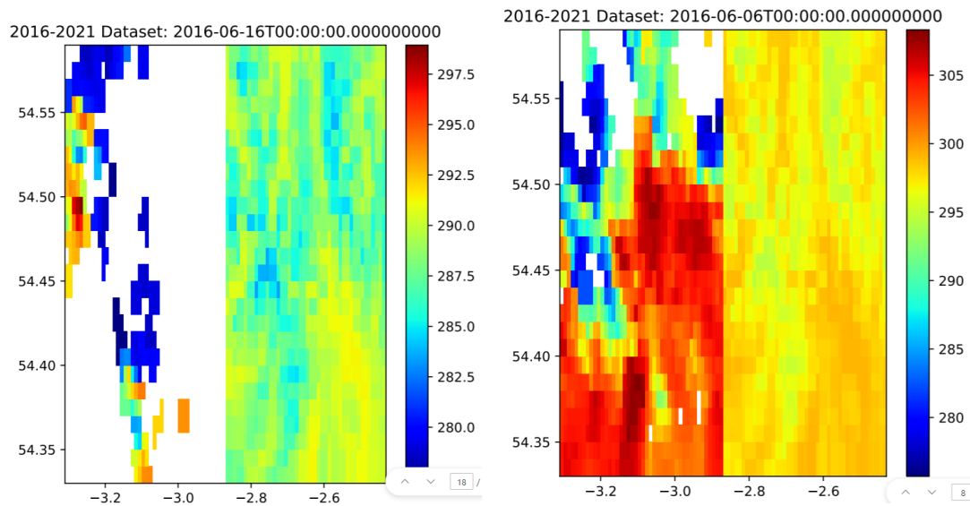
Figure 4-35: LST (left half of each image above) and maximum daily T2m from the HadUK-Grid dataset [RD-31] (right half of each image shown) showing data scarcity (white space) and cloud contamination (cold temperatures shown in blue) in the LST data.
