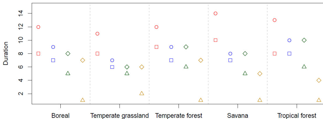
Figure 8 : Mean fire duration (in days) per fire patch for each biome (Boreal, Temperate grasslands, temperate forests, savannas and tropical forests) and for each dataset FRYv2 FireCCI51 (red), FRYv2 MCD64A1 (blue), FRYv1 MCD64A1 (green) and FRYv1 FireCCI41 (brown). Temporal cut-off thresholds for pixel aggregation are 6 days (square), 12 days (circle), 5 days (triangle) or 14 days (diamond).
