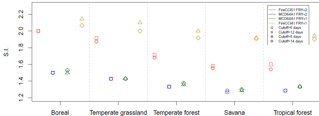
Figure 6: Mean shape index (S.I.) per fire patch for each biome (Boreal, Temperate grasslands, temperate forests, savannas and tropical forests) and for each dataset FRYv2 FireCCI151 (red), FRYv2 MCD64A1 (blue), FRYv1 MCD64A1 (green) and FRYv1 FireCCI41 (brown).
