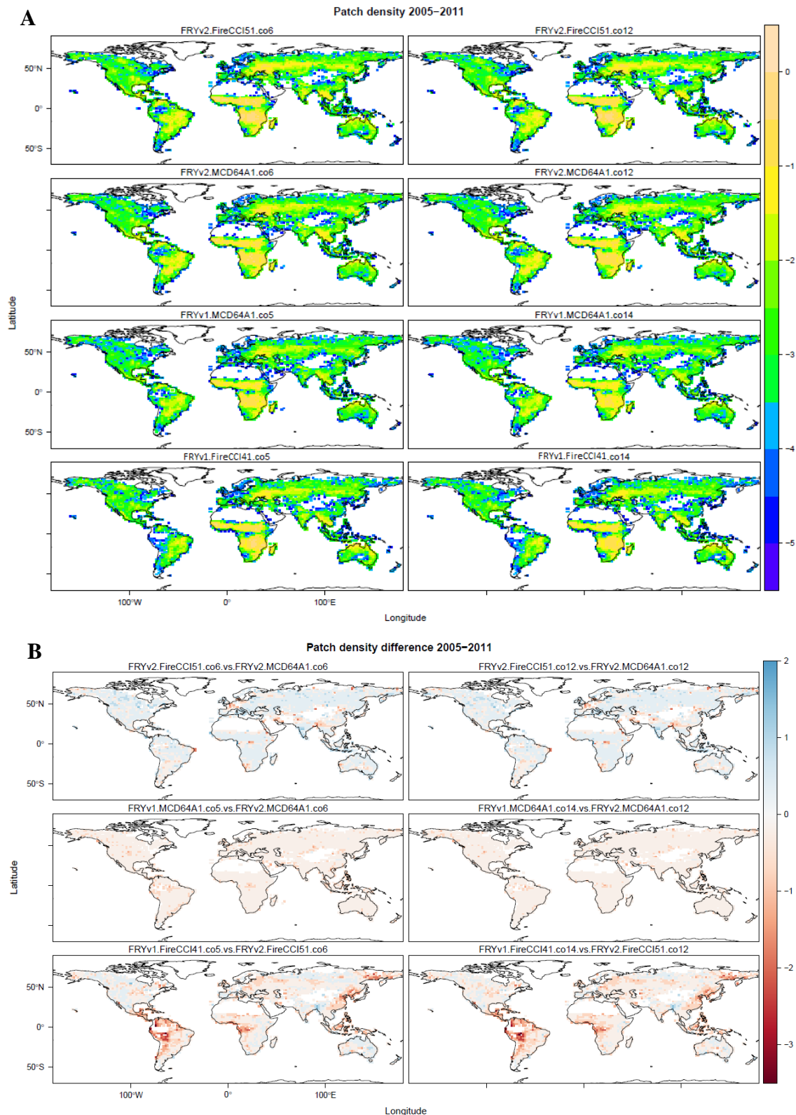
Figure 2: A) Global maps of fire patch density ( \log_{10}(\text{number of fires}) \cdot \text{km}^{-2} ) obtained for FRYv2 FireCCI51 (cut-off temporal threshold of 6 and 12 days), FRYv2 MCD6A1 (cut-off temporal threshold of 6 and 12 days), FRYv1 MCD64A1 (cut-off temporal threshold of 5 and 14 days), and FRYv1 FireCCI41 (cut-off temporal threshold of 5 and 14 days) over the 2005–2011 period. B) Global maps of fire patch density difference (in \log_{10}(\text{number of fires}) \cdot \text{km}^{-2} ) between FRYv2.0_FireCCI51 and FRYv2.0_MCD64A1, FRYv1.0_MCD64A1 and FRYv2.0_MCD64A1, and FRYv1.0_FireCCI41 and FRYv2.0_FireCCI51.
