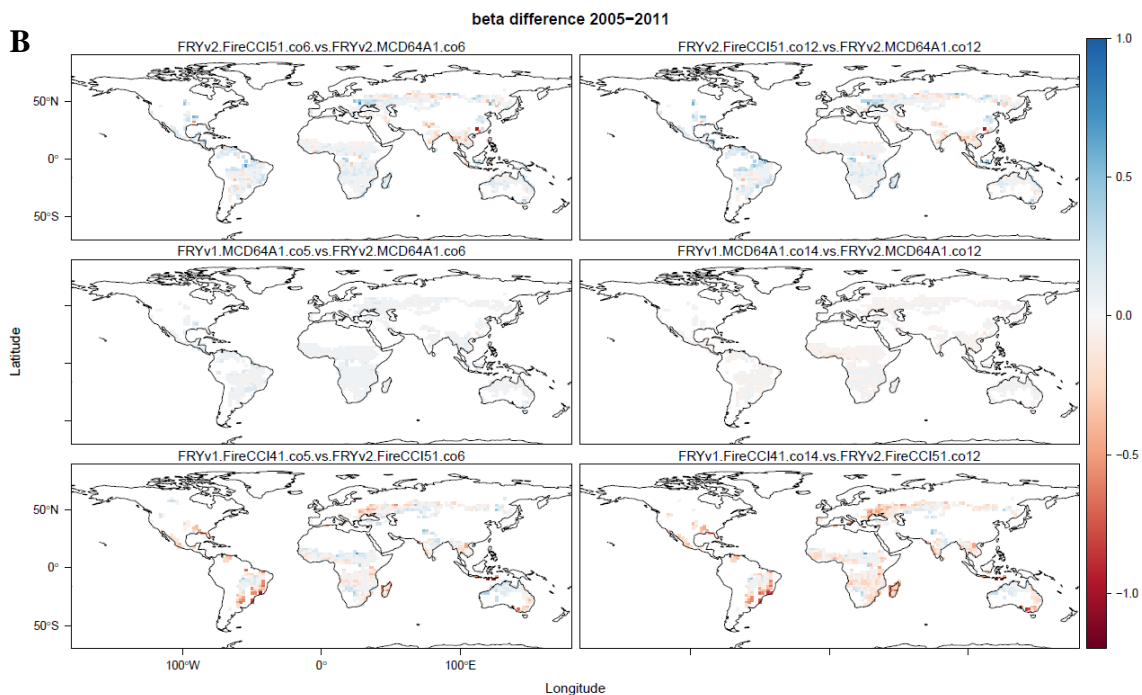
Figure 4: A) Global maps of fire size distribution slopes for fires >1000ha for FRYv2.0.FireCCI51, FRYv2.0.MCD64A1, FRYv1.0.MCD64A1 and FRYv1.0.FireCCI41 for temporal cut-off values of 6 days (left) and 12 days (right). B) Global difference maps between FRYv2.0.FireCCI51 and FRYv2.0.MCD64A1, FRYv1.0.MCD64A1 and FRYv2.0.MCD64A1, and FRYv1.0.FireCCI41 and FRYv2.0.FireCCI51.
