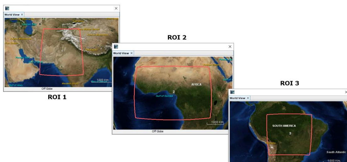
Figure 3-3: Regions of interest considered for TCWV high-resolution processing in WV_cci Phase 2.
