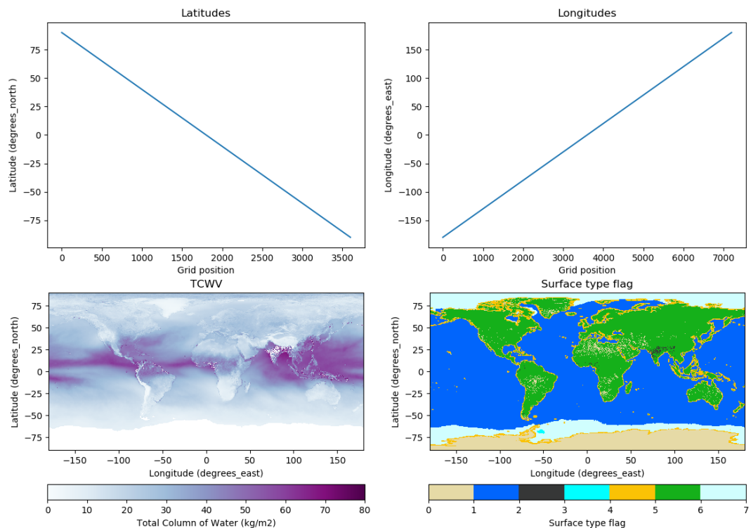
Figure 5-7: Result of applying the Python Matplotlib library to read and visualise TCWV data.
