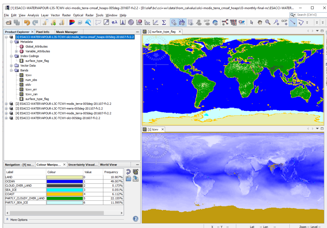
Figure 5-1: Visualising TCWV data with the SNAP Desktop application. See text for details.
