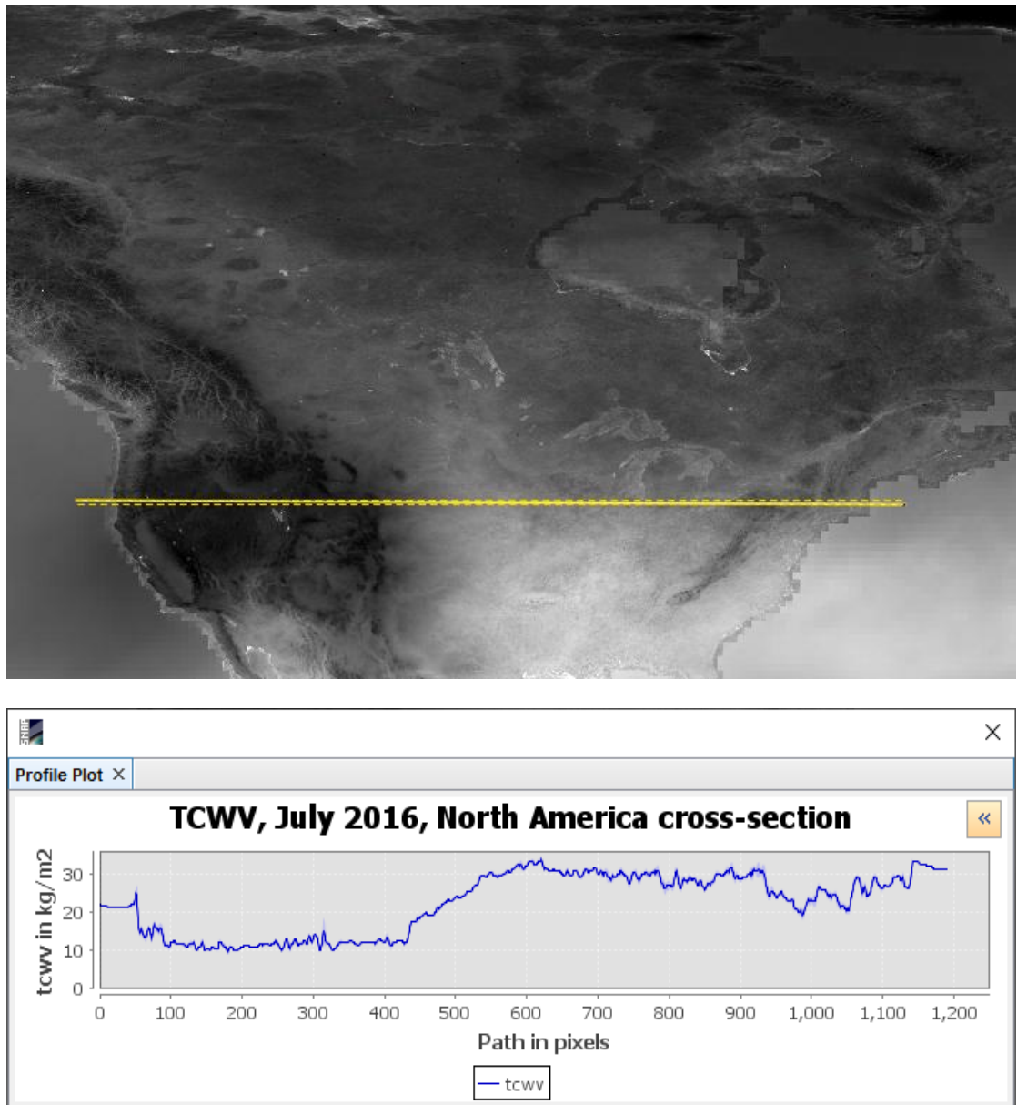
Figure 5-2: TCWV profile for a cross-section through North America.
