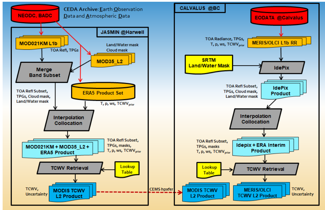
Figure 3-1: The TCWV L2 processing chains for MODIS Terra/Aqua, MERIS and OLCI A/B. See details in [4].
