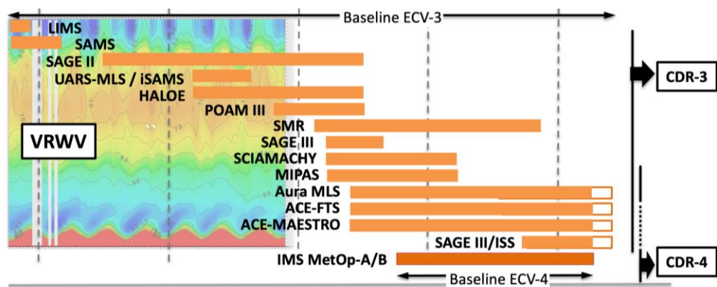
Figure 3-5: VRWV CDR-3 and CDR-4 input data and baseline.
