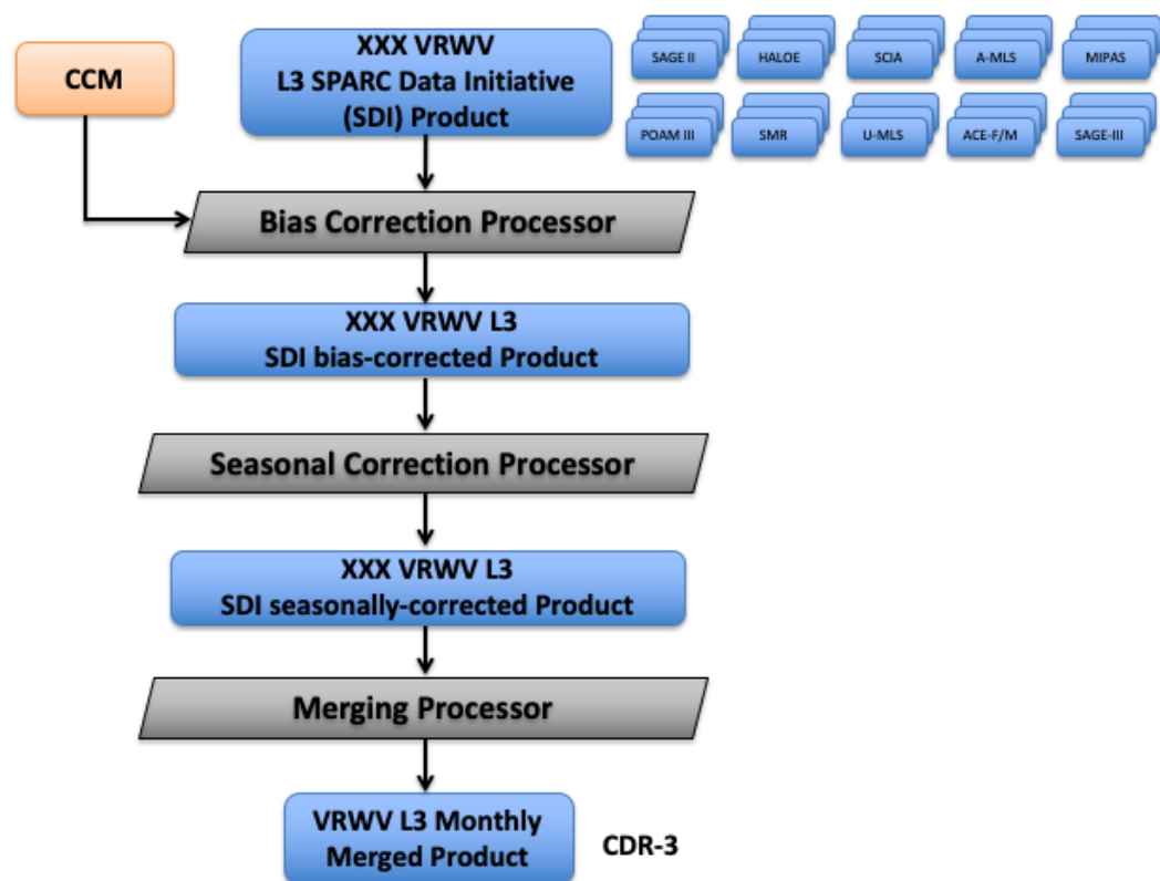
Figure 3-6: VRWV CDR-3 processing chain. See details in [4].
