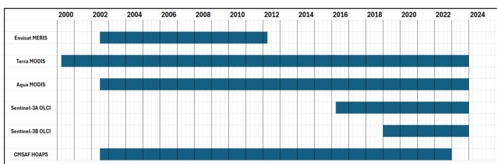
Figure 3-4: WV_cci Phase 2 TCWV instruments temporal coverage.
