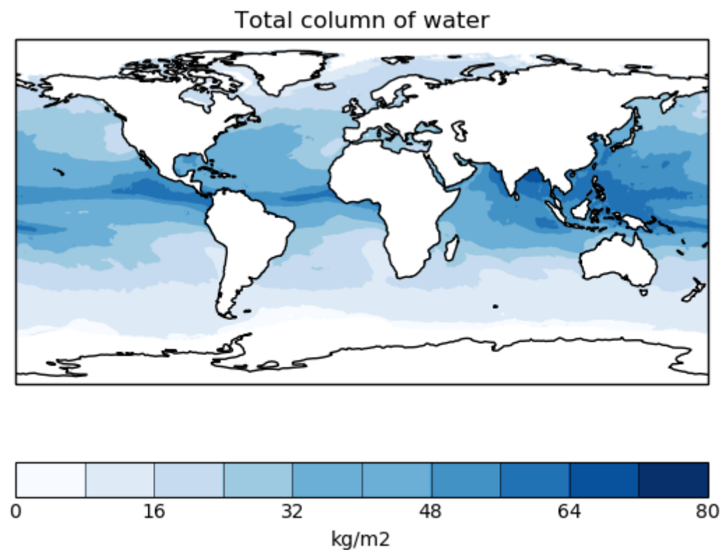
Figure 5-8: Result of applying the Python Matplotlib and Iris libraries to read and visualise TCWV data.
