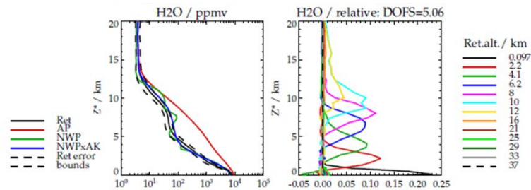
Figure 3-1: Retrieval diagnostics for water vapour for a mid-latitude scene over sea.
