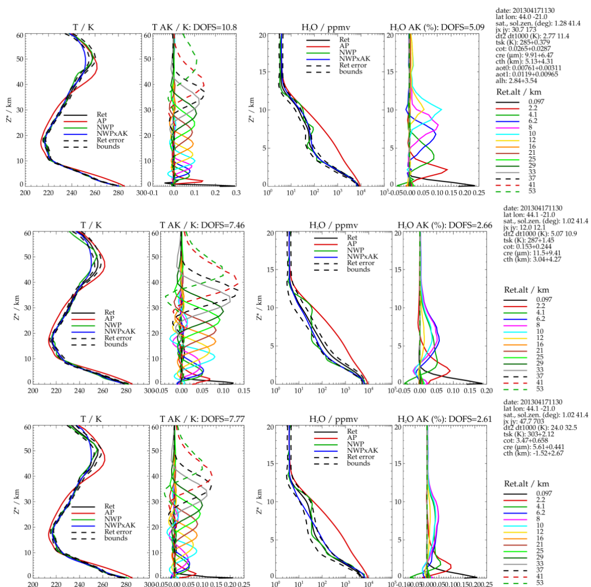
Figure 5-5 : Example retrieval output for mid-latitude cloud-free sea conditions. Upper set of panels show IASI results. Middle panels show results for a nearby comparable HIRS scenes, without using the SWIR channels (i.e only channels above 5 microns are used). Lower panels show results for HIRS scenes when all channels are used.
