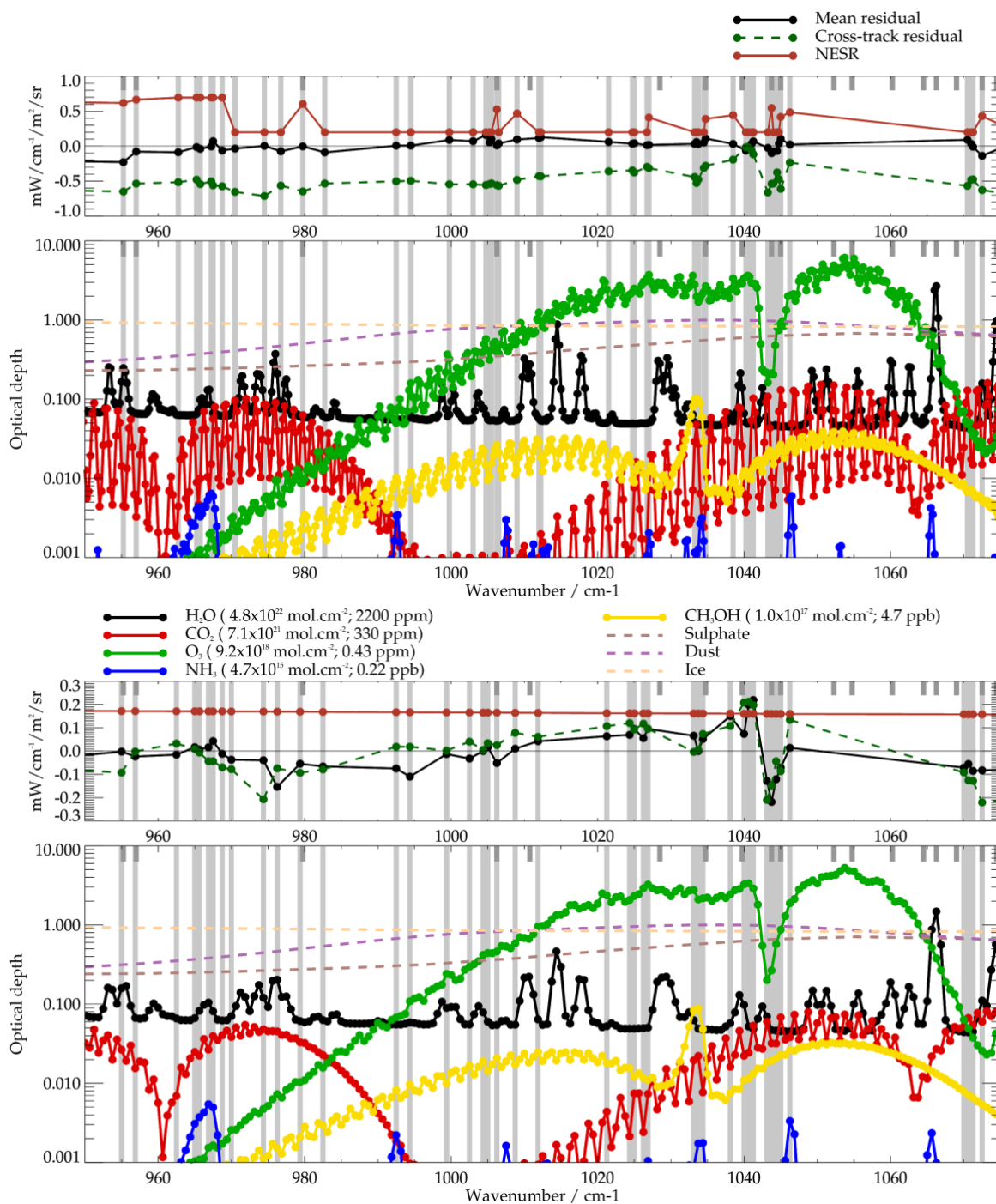
Figure 2-7 : Illustration of IMS spectral coverage, systematic residual spectral and assumed NESR, compared to trace gas and aerosol absorption spectra. Ozone and
