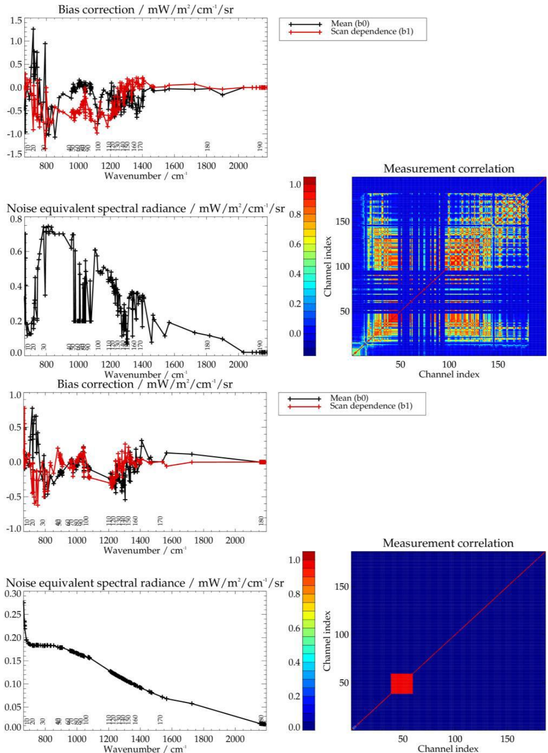
Figure 2-12 : Illustration of the IASI (upper panels) and CrIS (lower) bias correction and measurement error covariance. In each set of panels, the top left-hand panel shows the bias correction parameters. Numbers above the x-axis give the channel index from the subset used for the particular instrument. The bottom left panel in each set shows the estimated noise-equivalent spectral radiance, i.e. the square-root diagonal elements of the measurement covariance matrix. Bottom right shows the assumed measurement correlation matrix.
