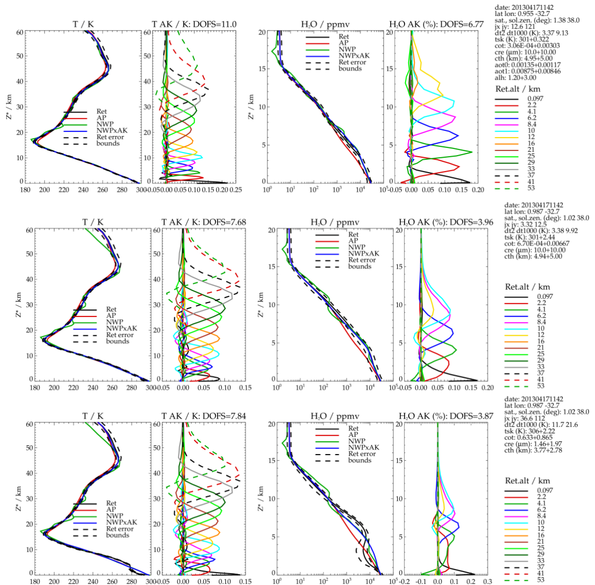
Figure 5-6 : Example retrieval output for tropical cloud-free sea conditions. Upper set of panels show IASI results. Middle panels show results for a nearby comparable HIRS scenes, without using the SWIR channels (i.e only channels above 5 microns are used). Lower panels show results for HIRS scenes when all channels are used.
