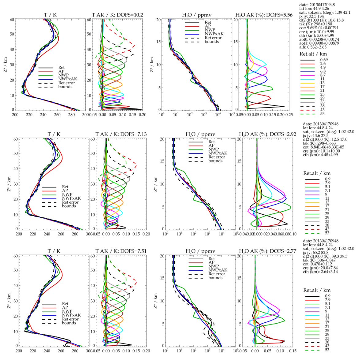
Figure 5-3 : Example retrieval output for mid-latitude cloud-free land conditions. Upper set of panels show IASI results. Middle panels show results for a nearby comparable HIRS scenes, without using the SWIR channels (i.e only channels above 5 microns are used). Lower panels show results for HIRS scenes when all channels are used.
