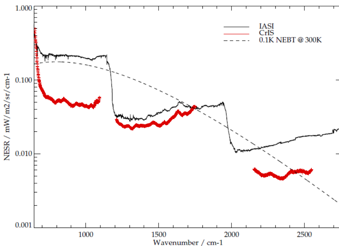
Figure 2-3: Comparison of spectral coverage and noise-equivalent spectral radiance (NESR) of IASI and CrIS. For comparison the dashed lines shows the NESR corresponding to 0.1 noise equivalent brightness temperature (NEBT) for a black body at 300K.
