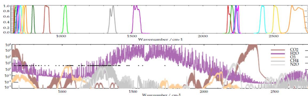
Figure 5-1 : Illustration of Metop B HIRS/4 channel spectral response functions (middle panel), compared to the main gas optical depths at IASI spectral resolution (lower panel). Black dots along the middle of the lower panel indicate the IASI channels normally used by IMS.
