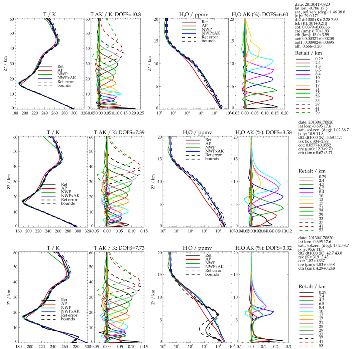
Figure 5-4 : Example retrieval output for tropical cloud-free land conditions. Upper set of panels show IASI results. Middle panels show results for a nearby comparable HIRS scenes, without using the SWIR channels (i.e only channels above 5 microns are used). Lower panels show results for HIRS scenes when all channels are used.
