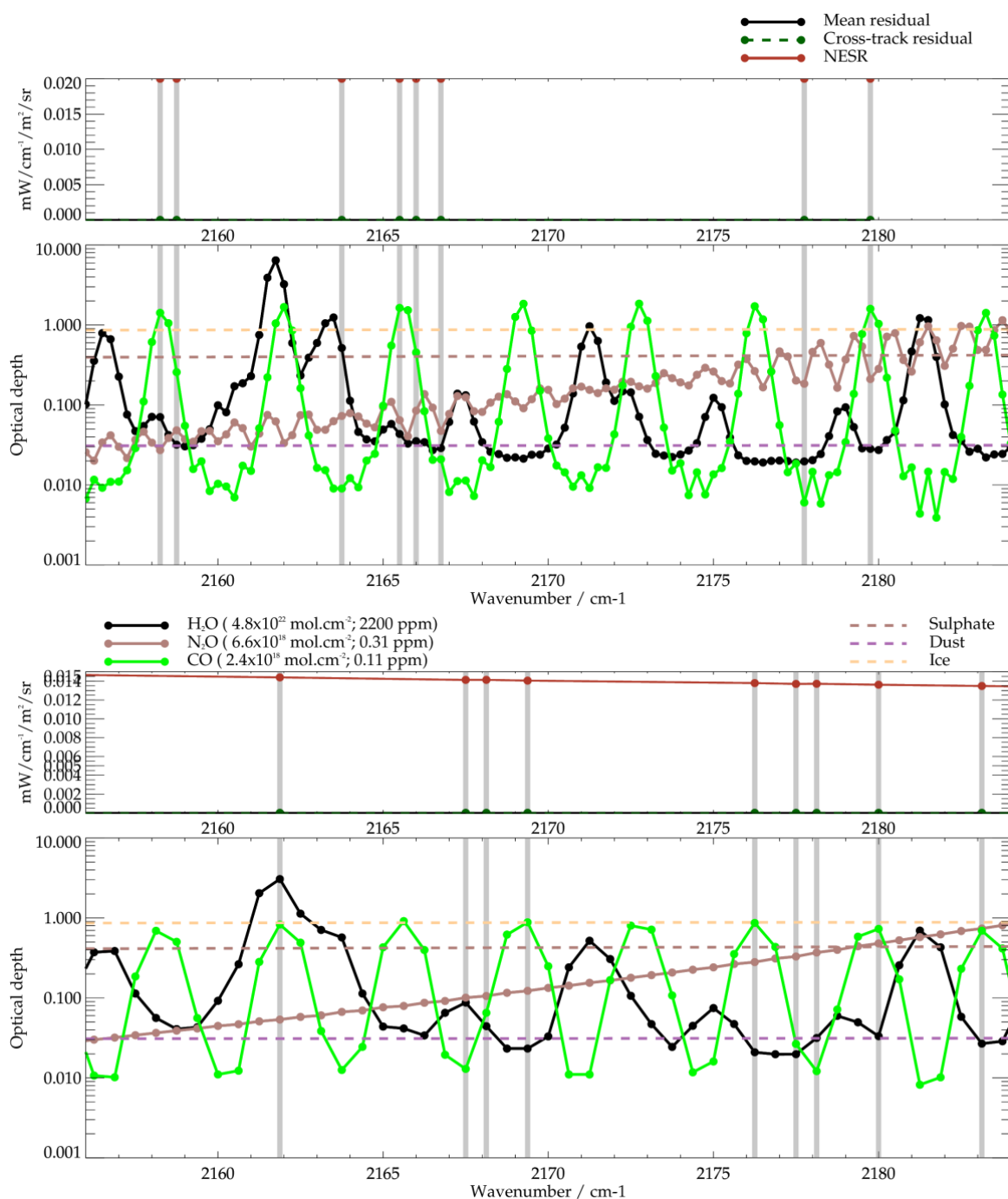
Figure 2-11 : Illustration of IMS spectral coverage, systematic residual spectral and assumed NESR, compared to trace gas and aerosol absorption spectra. Carbon monoxide spectral range from 2156 - 2184 cm -1 . Upper pair of panels are for IASI; lower pair of panels are for CrIS. Light grey vertical bars indicate the spectral channels used by IMS-extended. Channels used by the previous IMS-v1 scheme are indicated by the smaller dark bars towards the top of each sub-panel.
