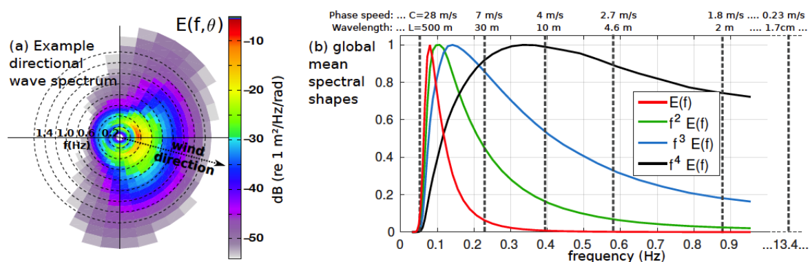
Figure 1: (a) example of wave spectrum E(f, \theta) that represents the distribution of the surface elevation variance across wave frequencies and directions, obtained from stereo-video imagery (Leckler et al. 2015) (b) Spectral shapes of global averages distributions of elevation E(f) , wave-induced velocities f^2 E(f) , Stokes drift f^3 E(f) – this simplified expression assumes all waves propagate in the same direction – and acceleration f^4 E(f) , which is proportional to surface slope in the case of linear waves. Each spectrum was normalised by its maximum value.
