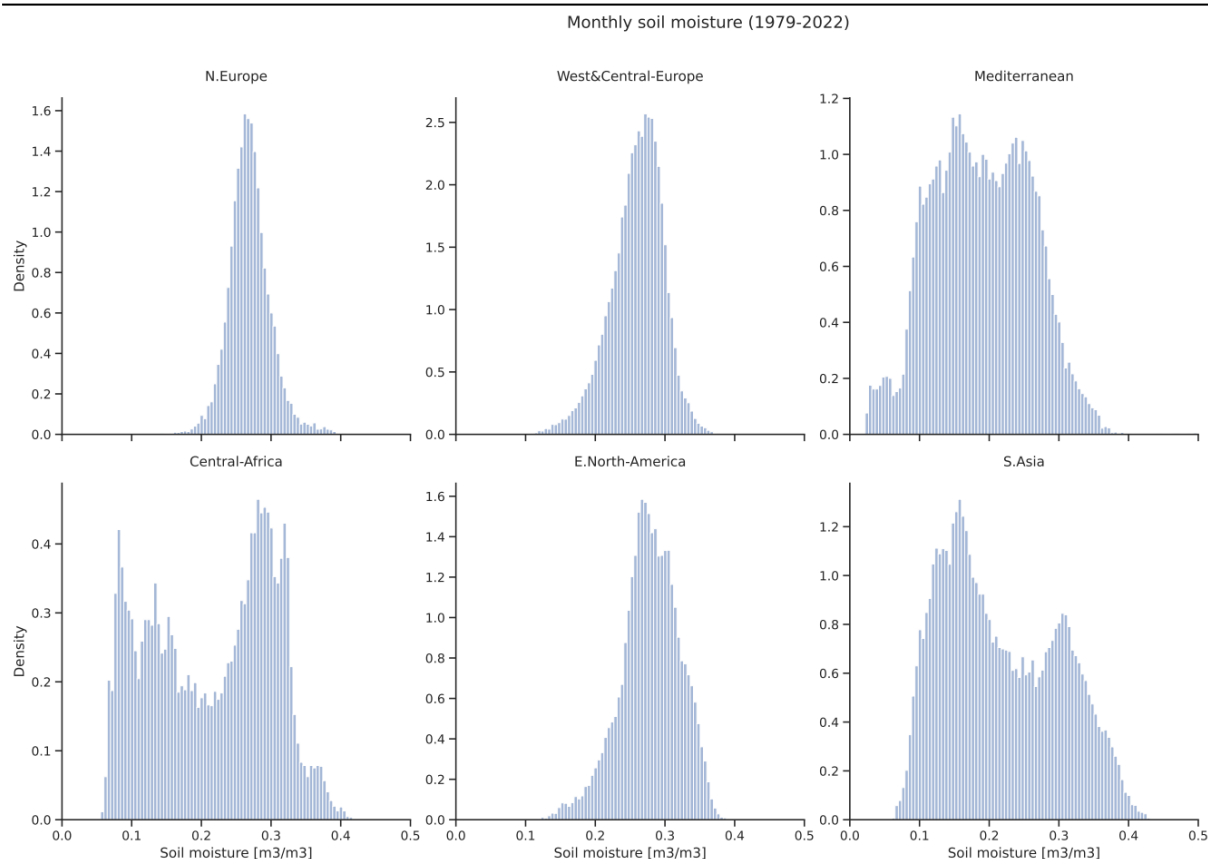
Figure 12 Spatiotemporal distribution of monthly mean soil moisture from ESA CCI SOILMOISTURE in the period 1979-2022 for six IPCC AR6 regions (from left to right) northern Europe, West & Central Europe, Mediterranean Europe, Central Africa, eastern North America and South Asia. Each month in each grid cell in the corresponding regions is considered with equal weight.
