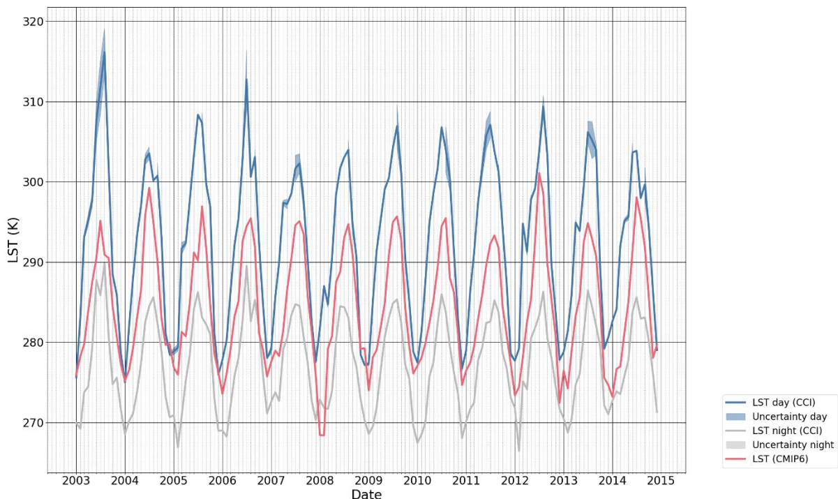
Figure 19 The LST_cci and calculated total uncertainty, and model comparison. The daytime and night-time overpasses from the LST_cci are given in blue and grey respectively, with shaded regions showing \pm 1 total uncertainty as in Figure 9. The red line is the land surface temperature from the model discussed in the text.
