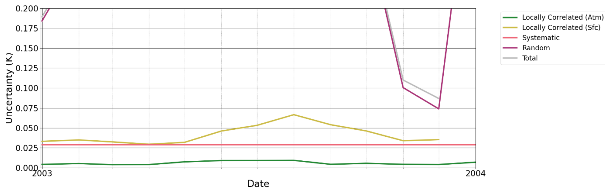
Figure 15 A zoom in on part of the daytime LST uncertainty values as propagated for the year 2003 and uncertainty values of less than 0.2 K. This shows the structure in both locally correlated components.
