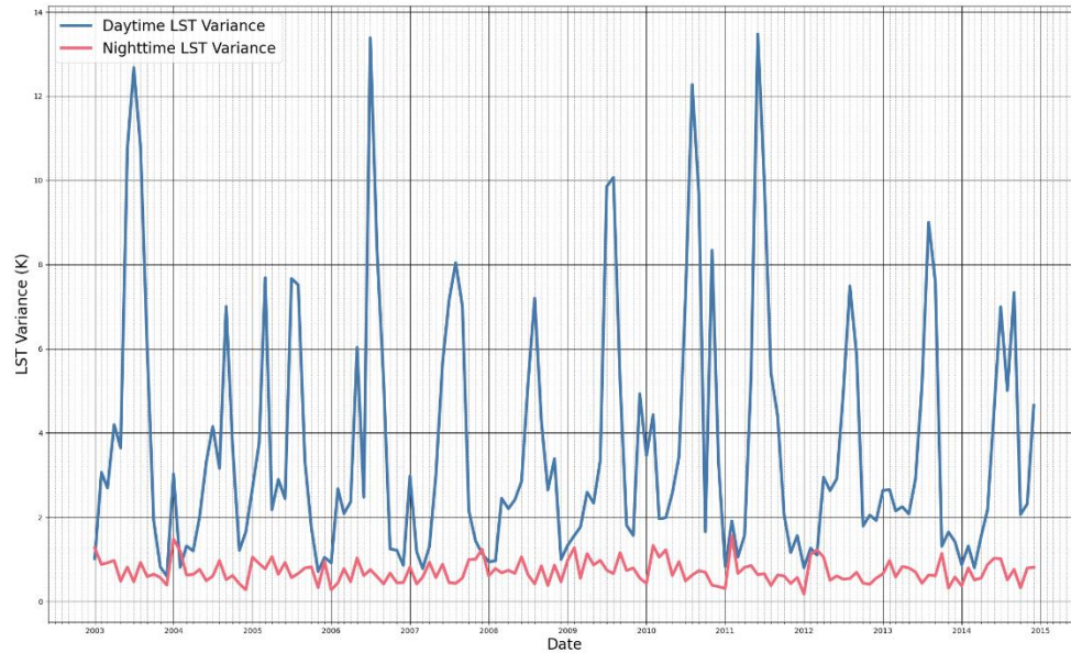
Figure 17 The land surface temperature (LST) variance of the daytime (blue) and night-time (red) overpasses for the region defined in the text. The daytime variance is seen to be large in the summer months. This affects the value of the propagated random uncertainty components at these times.
