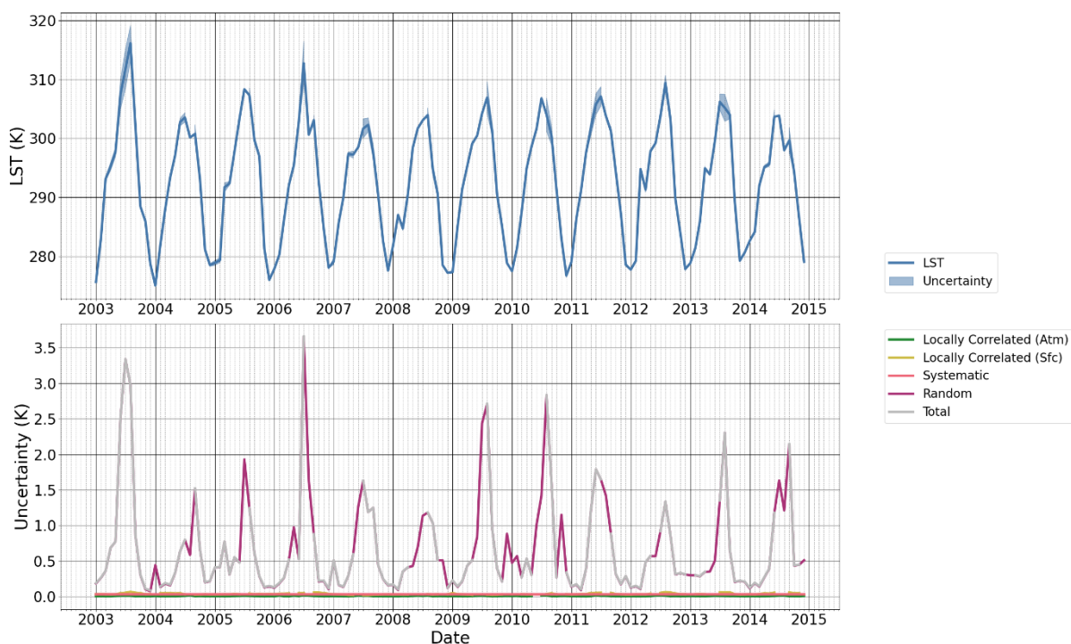
Figure 14 Timeseries plots of the daytime Land Surface Temperature (LST) and the propagated uncertainty components for the region of France defined in the text. (top) The mean LST shown with \pm 1 times the
