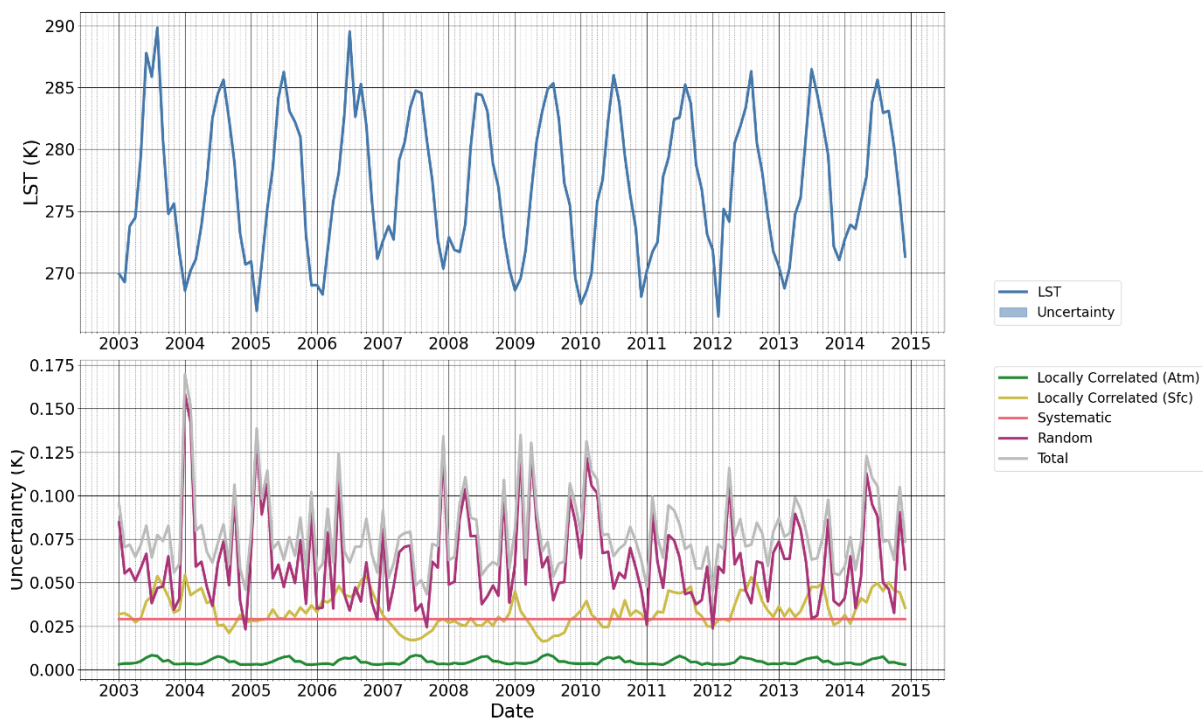
Figure 16 The same plots as in Figure 14 but for the night-time overpass data.
