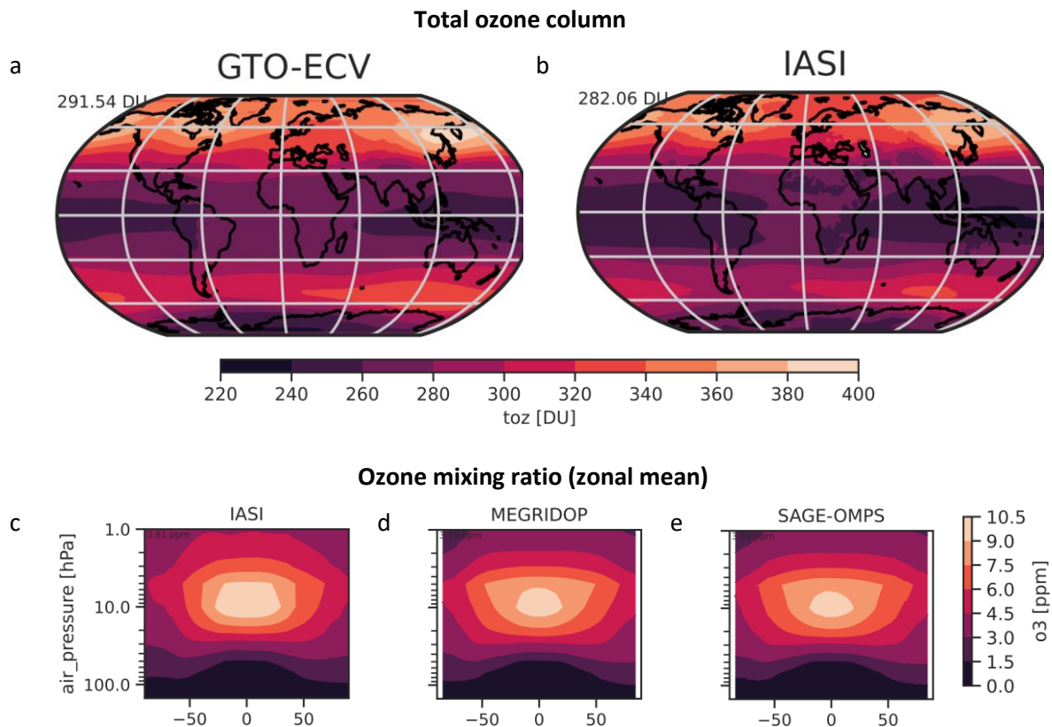
Figure 11 Multi-year (2008-2022) annual average (top) total column ozone in Dobson Units (DU) and ozone mixing ratio in ppm from ESA CCI OZONE. (a) GTO-ECV, (b, c) IASI, (d) MEGRIDOP, (e) SAGE-OMPS.
