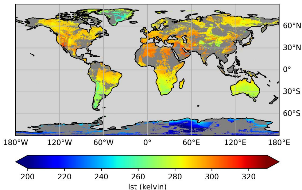
Figure 14: Example of NOAA19_AVHRR_L3C_0.05 daily descending data for 31 st July 2007. This product collates several orbits in each file. Cloud masking has been applied to this data.
