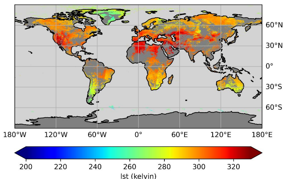
Figure 13: Example of Metop-A_AVHRR_L3C_0.01 daily daytime data for 31 st July 2020. This product collates several orbits in each file. Cloud masking has been applied to this data.
