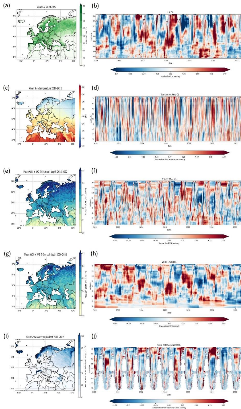
Figure 2: ISBA simulations over Eurasia forced by ERA5 atmospheric variables from 2010 to 2022 at a spatial resolution of 0.25^\circ \times 0.25^\circ . Mean values (a,c,e,g,i) and Hovmöller plot (b,d,f,h,j) of scaled anomalies of (a,b) LAI, (c,d) LST, (e,f) surface soil moisture, (g,h) deep soil moisture (0.8-1.0m), (i,j) SWE.
