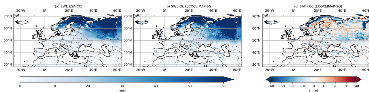
Figure 5: Map of mean SWE value over Eurasia from (a) CCI Snow, (b) ISBA open-loop simulations feature 2b (Table 1), and (c) the difference between CCI Snow and ISBA open-loop simulations feature 2b (Table 1).
