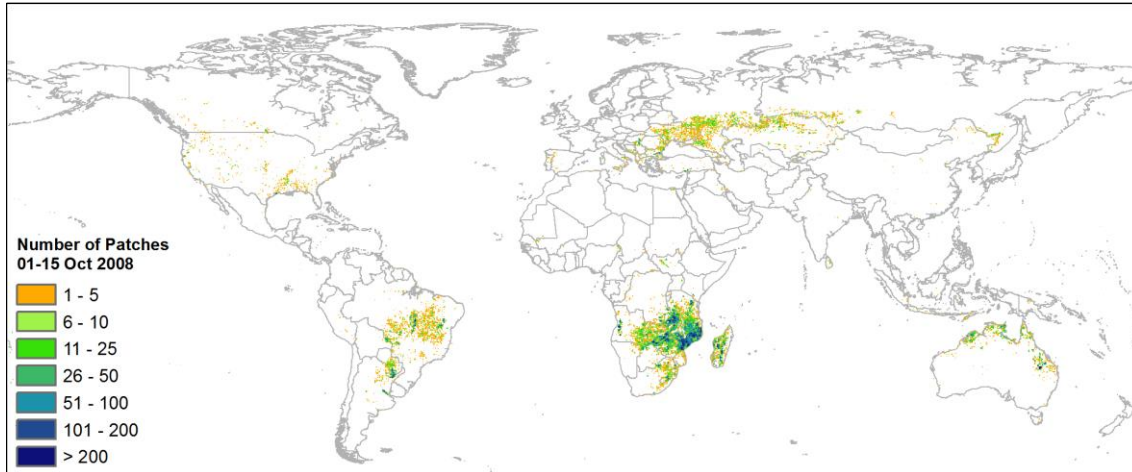
Figure 3.5: Example of the Number of Patches attribute of the 20081007-ESACCI-L4_FIRE-BA-MERIS-fv04.1.nc file.
