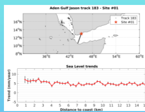
examples of coastal sea level trends (2002-2020) from retracked Jason-1, 2, 3 Upper panel: location of the Jason track (black line) and of the virtual station (red star) Lower panel: sea level trend computed over 2002-2020 against distance to the coast
