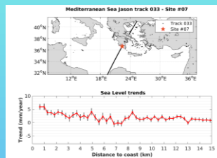
examples of coastal sea level trends (2002-2020) from retracked Jason-1, 2, 3 Upper panel: location of the Jason track (black line) and of the virtual station (red star) Lower panel: sea level trend computed over 2002-2020 against distance to the coast
