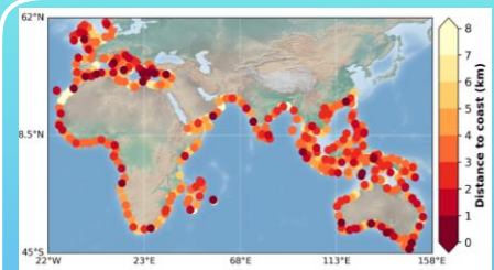
Closest distance (km) to the coast of the first valid point along the Jason track for all 756 virtual stations (distance to coast < 6 km)
