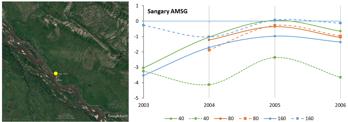
Figure 4.12 Left Panel: Yellow point=Locality of Sangary AMSG (Dataset 24652 from RHM, Long 127.46, Lat 63.96), Map source: Google Earth Pro ©, Version 7.3.2. Right panel: MAGT of site Sangary AMSG for depths of 40, 80 and 160 cm. Solid lines= in situ mean MAGT [°C], broken lines= Permafrost_cci mean MAGT [°C] of CRDPv0. The deviation of Permafrost_cci and in situ MAGT data varies both, between depths and between years (mean bias -0.27 °C, SD of bias 1.86 °C).
