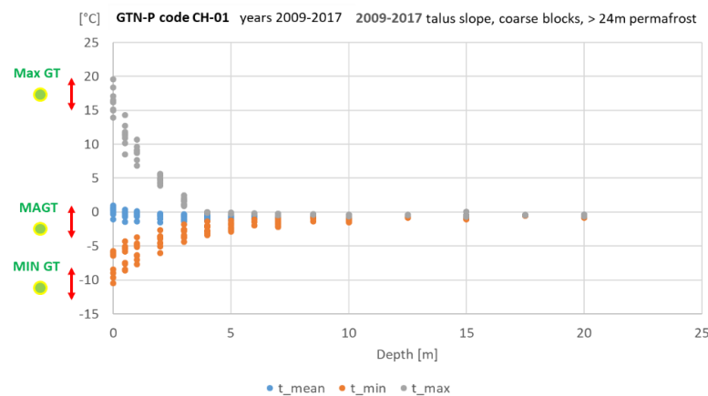
Figure 4.10: High inter-annual variability of MAGT, min annual GT and max annual GT in mountain permafrost
