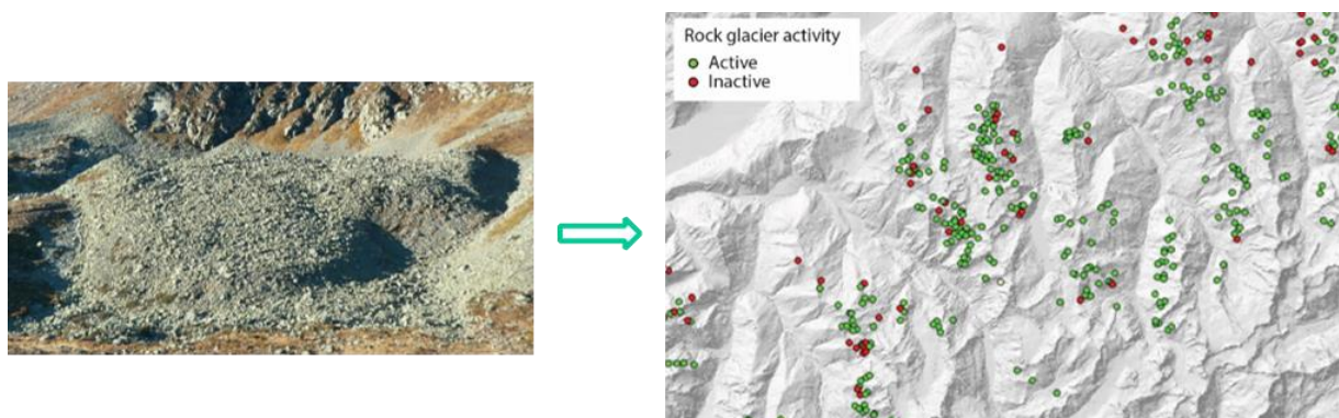
Figure 4.16: Example of typical rock glacier (left panel) and rock glacier inventory in the Swiss Alps, which includes the state of activity of each landform (right panel).
