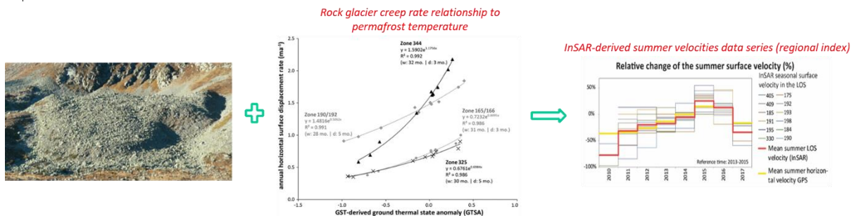
Figure 4.17: Schematic representation of the proposed regional kinematic indices computation.
