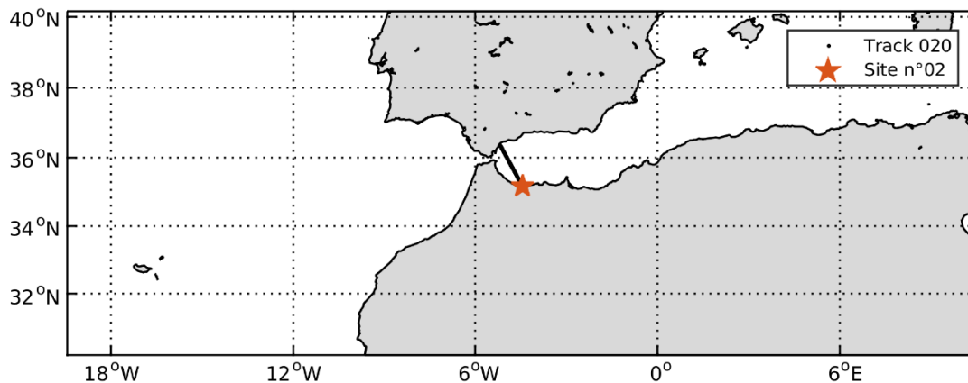
Sea Level trends
