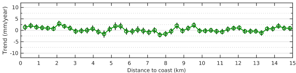
Sea Level trends
